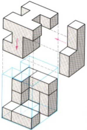
Fig. 11 Orthographic projections of a 3D object with a cut section
