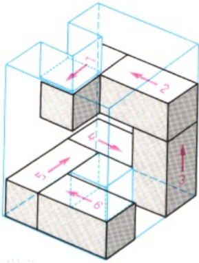
Fig. 10 Orthographic projections of a 3D object
